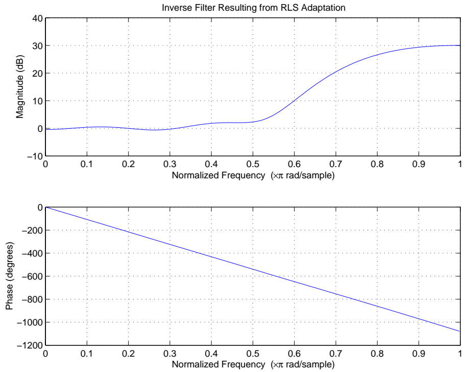
Figure 4-2: After Adapting, the RLS Algorithm Produces a Highpass Filter
